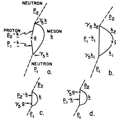
FIG. 10. According to the meson theory a neutron interacts with an electromagnetic potential \mathbf{a} by first emitting a virtual charged meson. The figure illustrates the case for a pseudoscalar meson with pseudovector coupling. Appendix D.
