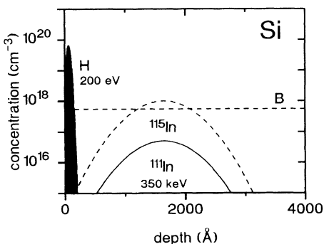
FIG. 3. Depth profiles of impurity concentrations for typical samples: The ^{111}\text{In} probe atoms are implanted at 350 keV (solid line). H loading with 200-eV implantation energy (here, 5 \times 10^{13} \text{ cm}^{-2} ) leads to a shallow H profile (black) so that H has to diffuse into the sample to form In-H pairs. Several experiments were performed using higher p -type doped material (dashed lines), e.g., either homogeneous B-doped (here, 5.5 \times 10^{17} \text{ cm}^{-3} ) or additionally implanted with stable ^{115}\text{In} (peak concentration 10^{18} \text{ cm}^{-3} ).
